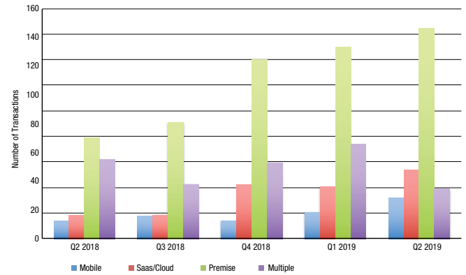
Chart 13: Software Deployment Channels
